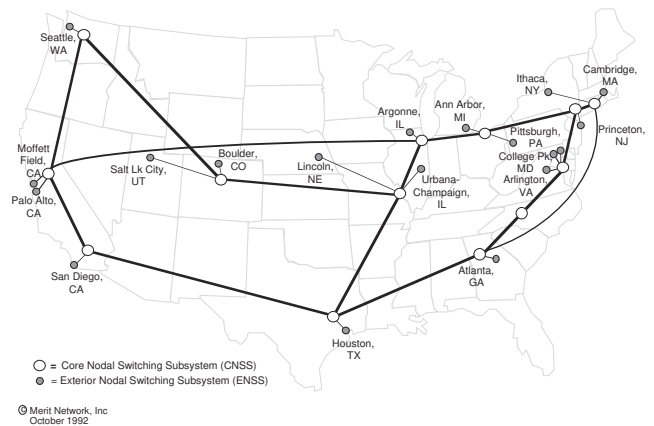
Figure 1: 1992 NSFNET T3 Backbone Service Logical Topology
