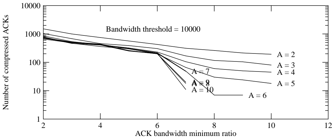
Figure 9: Sensitivity of ACK-compression analysis (minimum bandwidth held constant)
